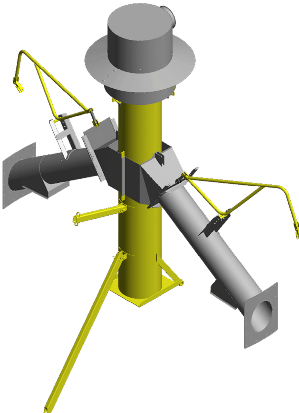
Tubo e coclea con aspirazione – Extension tube with auger and aspiration head
