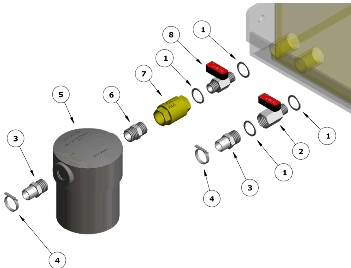
FIG. 11 Raccorderia – Connections
