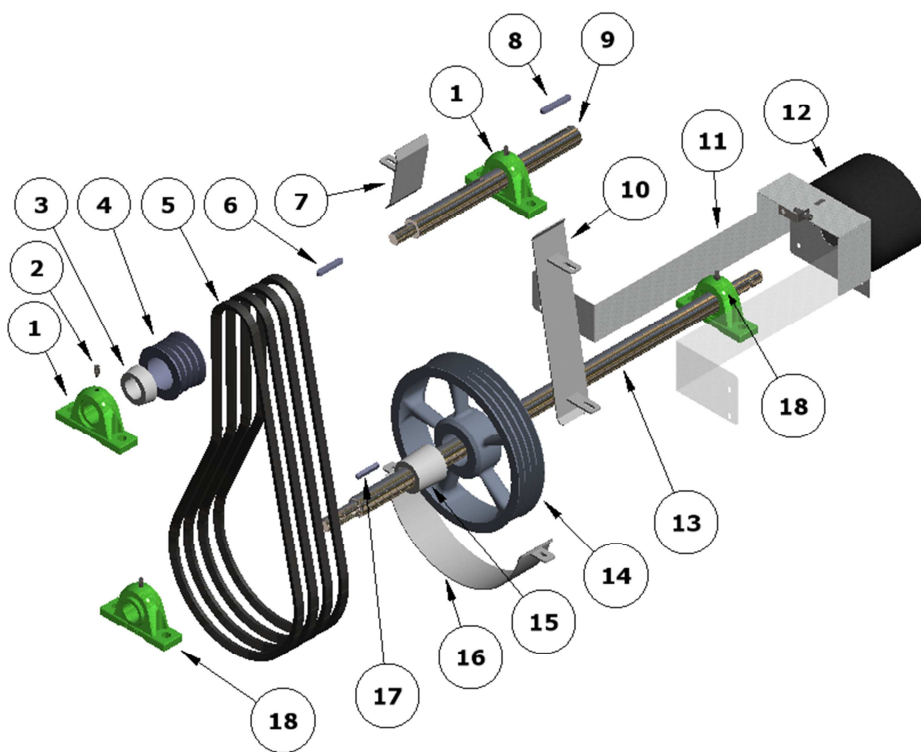
FIG. 7 Trasmissione del ventilatore - Transmission of the fan
